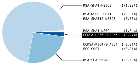
Fig. 3. Use of DNSSEC algorithms in .com on August 31, 2016
